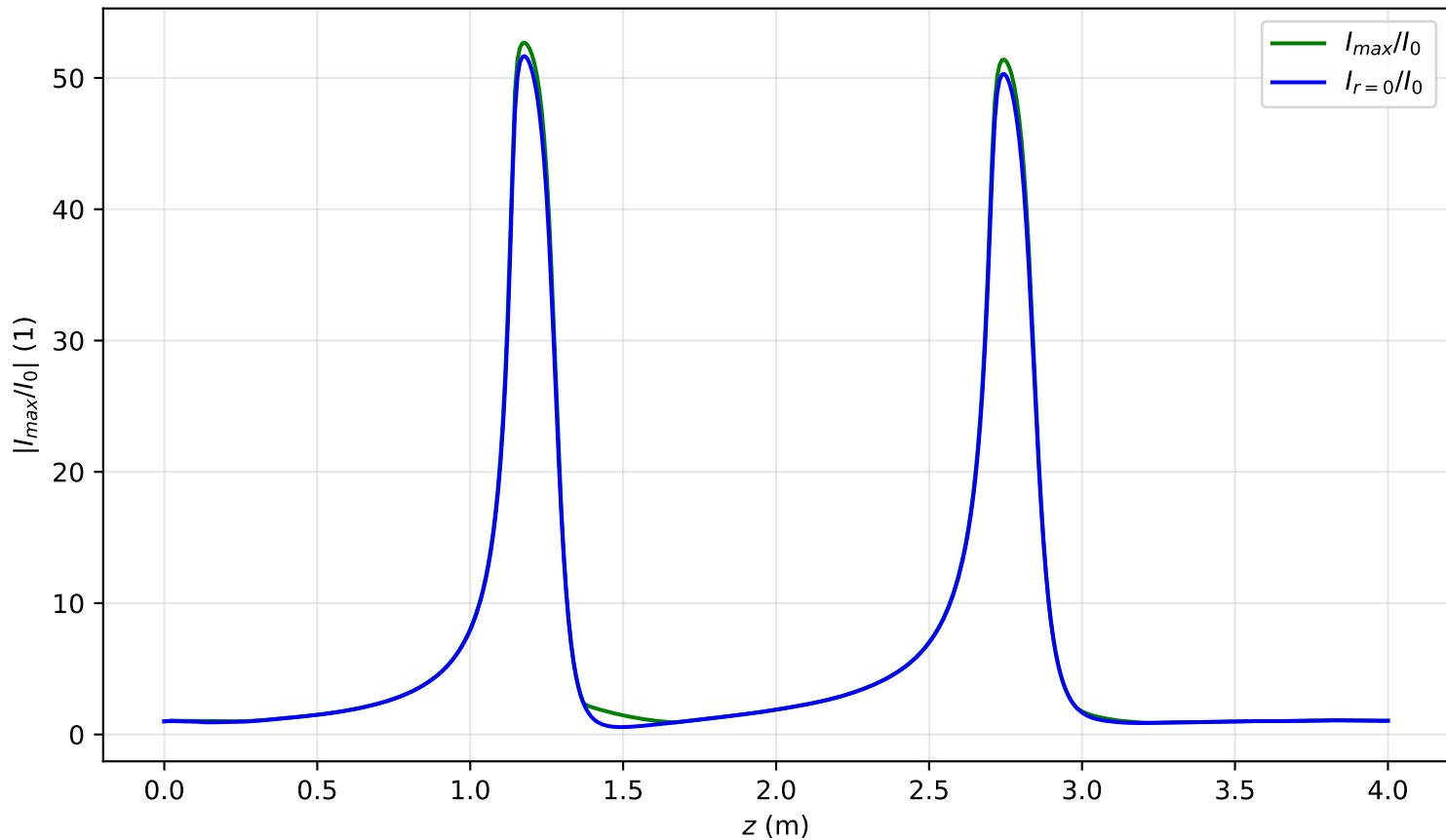
I_{max}(x=0, y=0, z)/I_0 , P_{in}=2.0P_{cr} , noisy input, artificial time
